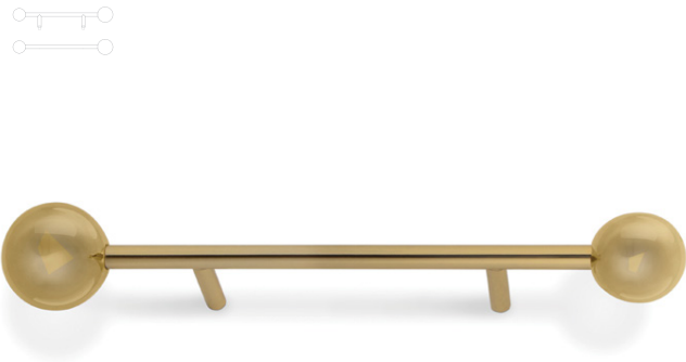
TW5005 Door Hardware - Door Pull H 270 mm | 10,63" L 43 mm | 1,69" D 56 mm | 2,20"
